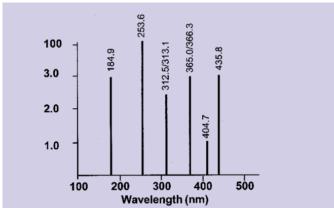
MERCURY SPECTRUM
