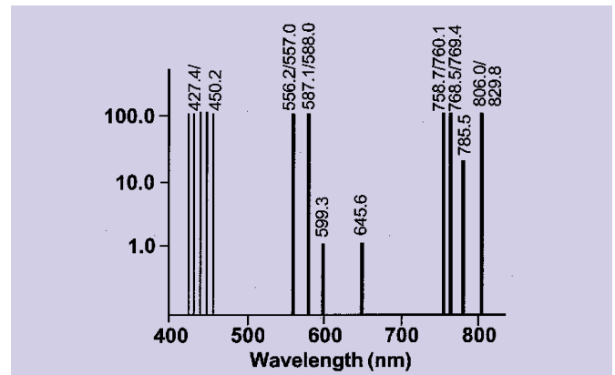
KRYPTON SPECTRUM
