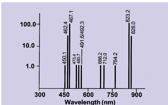
XENON SPECTRUM
