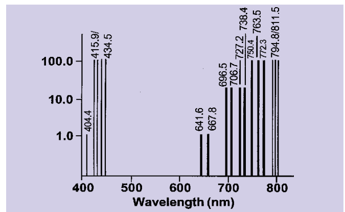
ARGON SPECTRUM
