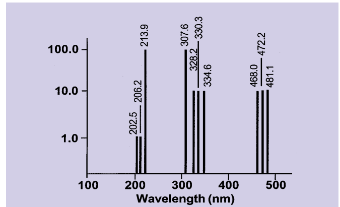
ZINC SPECTRUM
