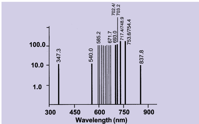
NEON SPECTRUM
