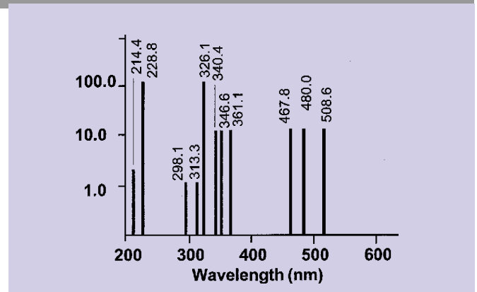
CADMIUM SPECTRUM
